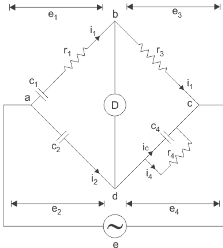
Schering Bridge
