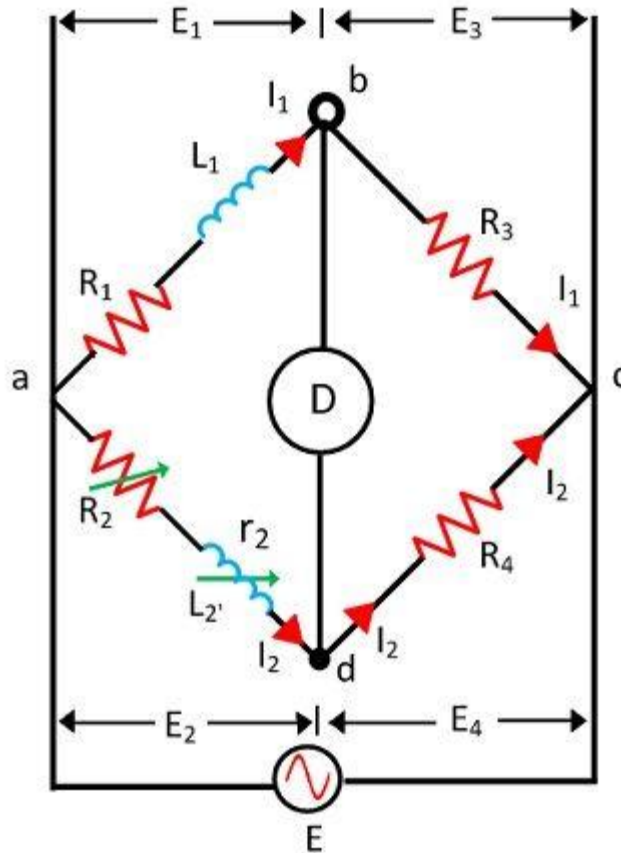
Maxwell's Inductance Bridge
