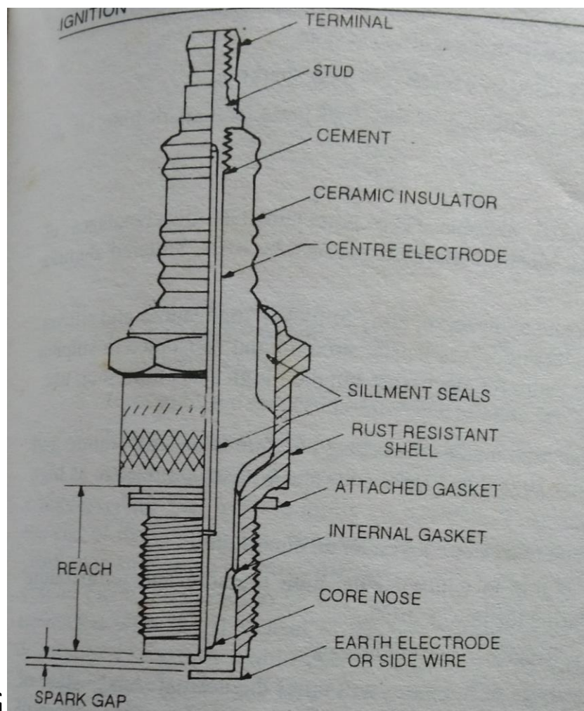
SPARK PLUG
